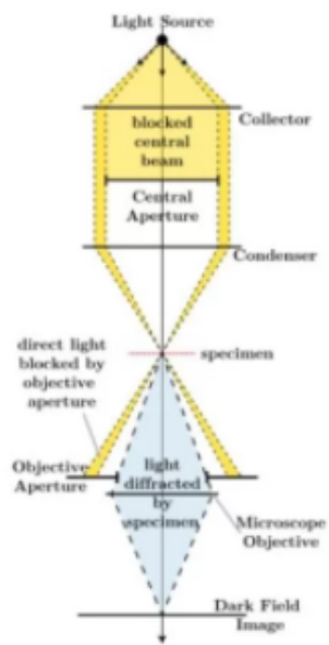
Figure 76.2 Working Principle of Dark Field Microscopy
