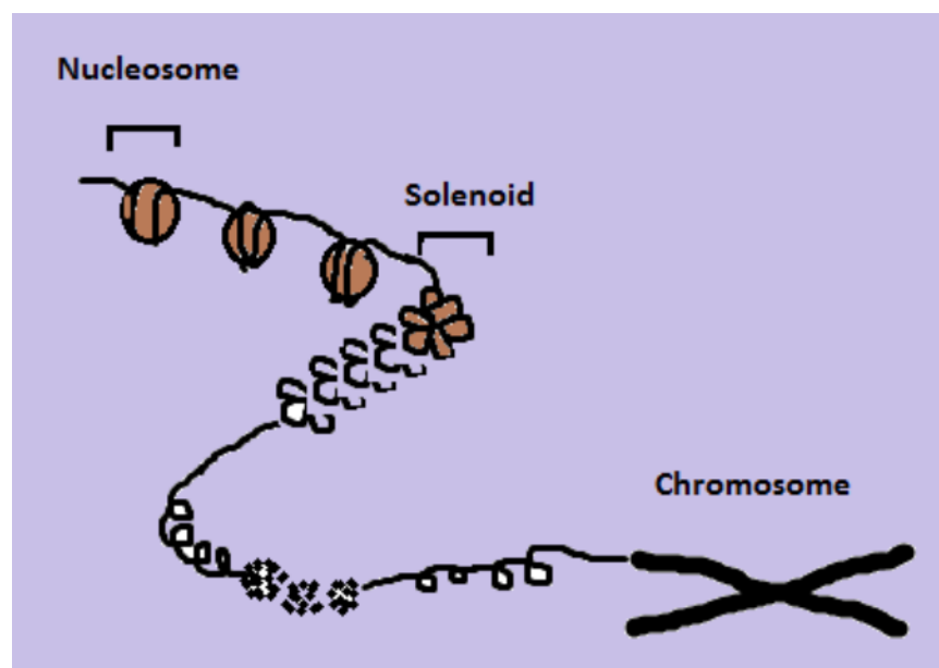
Figure 24.1 Chromosome coiling and nucleosome
