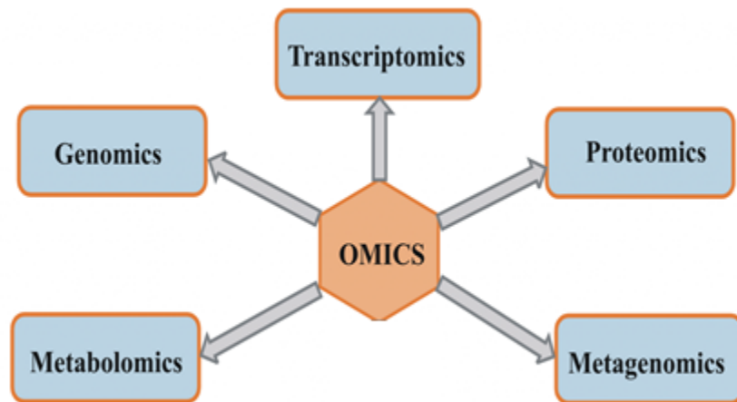
Figure 37.1 Important branches of Omics
