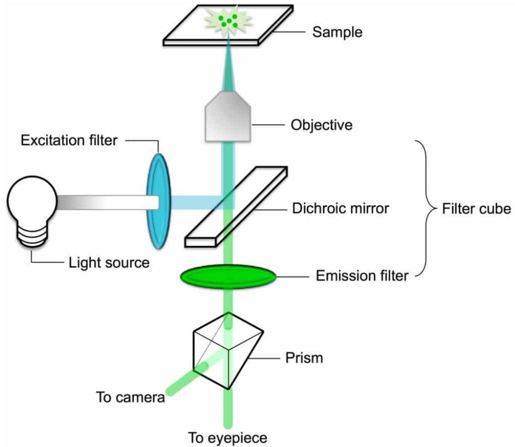
Figure 76.5 Principle of fluorescent microscopy
