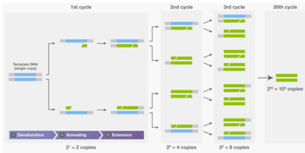
Figure 44.1 Three steps of PCR—denaturation, annealing, and extension—as shown in the first cycle, and the exponential amplification of target DNA with repeated cycling.
