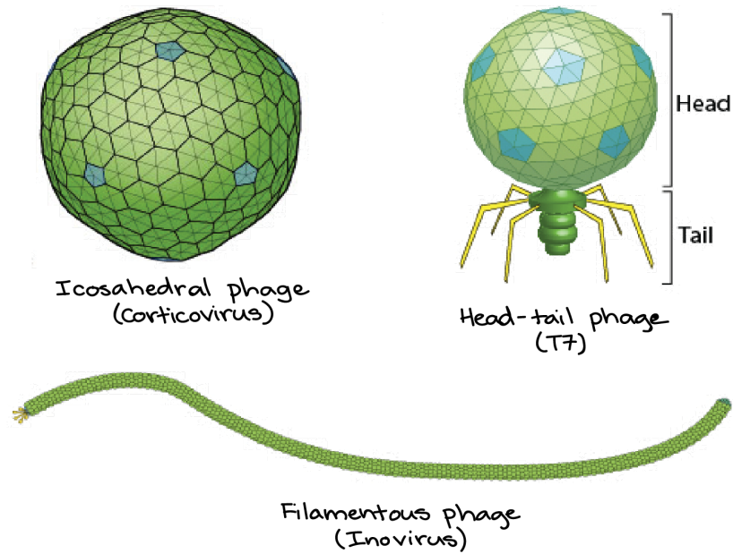
Figure 70.1 Icosahedral phage, head-tail phage, and filamentous phage
