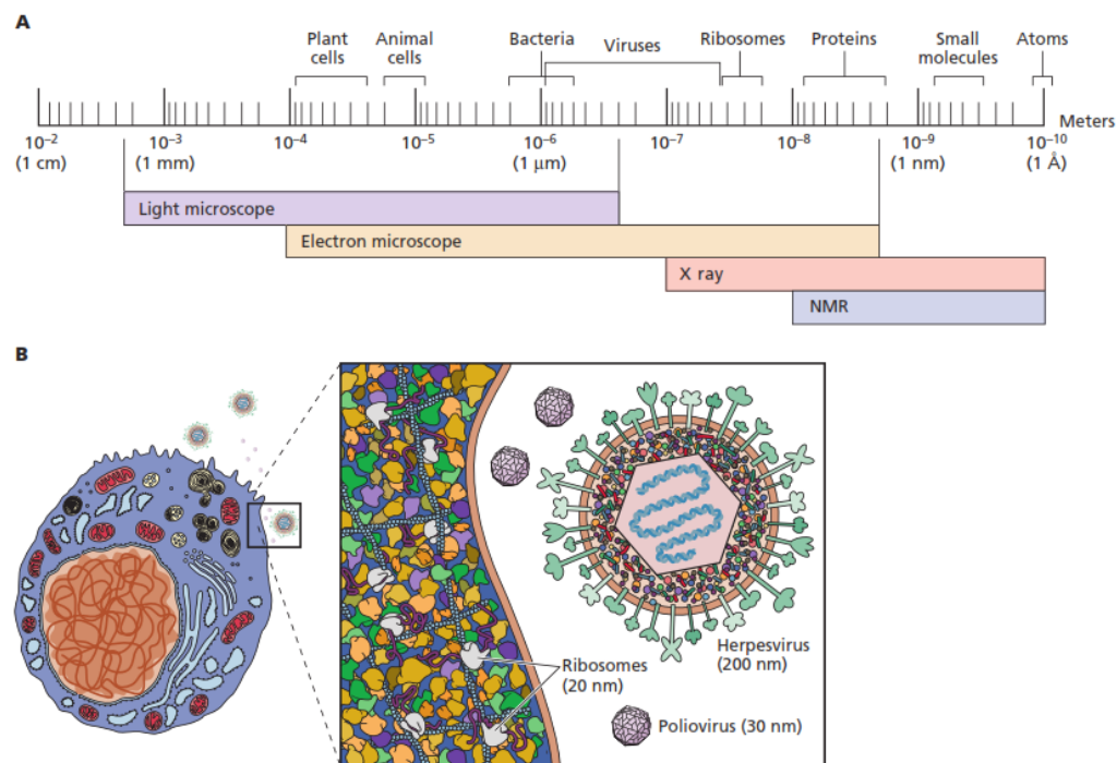
Figure 66.1 (A) Sizes of animal and plant cells, bacteria, viruses, proteins, molecules, and atoms are indicated. The resolving powers of various techniques used in virology, including light microscopy, electron microscopy, X-ray crystallography, and nuclear magnet
